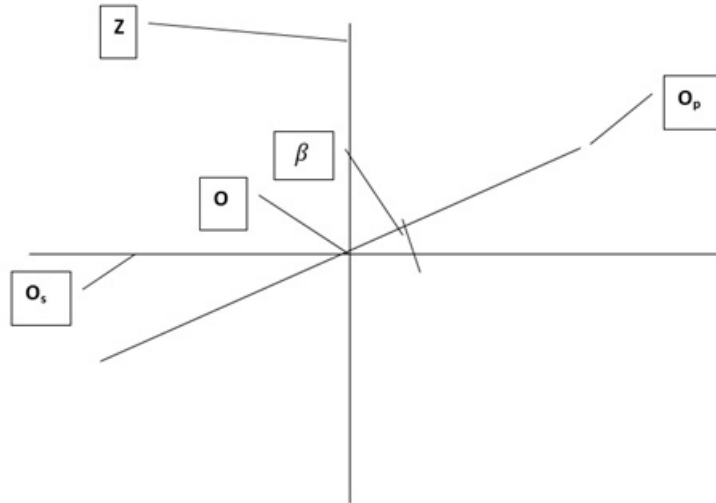
Figure 1: Cross section of the solar system.
